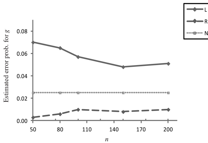
FIGURE 3. Estimated error probabilities for g at \alpha = 0.05
